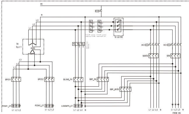
STS100D CABINET
